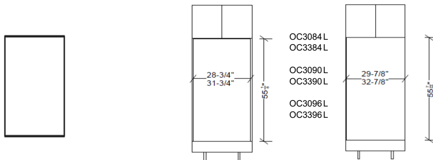
Oven Cabinet (Double) shown without Trim Kit
